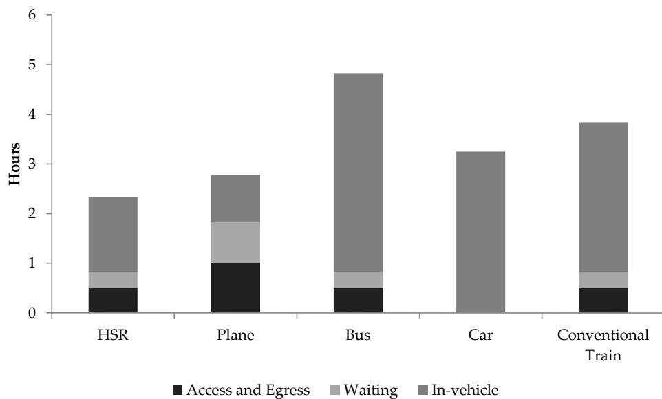
Figure 11. Door-to-door trip time (Madrid-Zaragoza)
